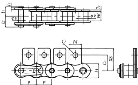
SA1 Attachment
