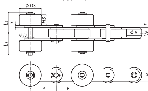
Crosswise Installation (Type II)
