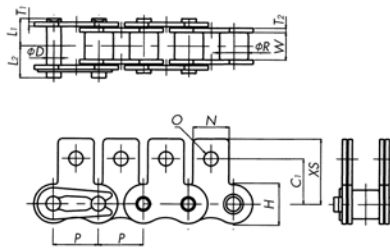
SK1 Attachment
