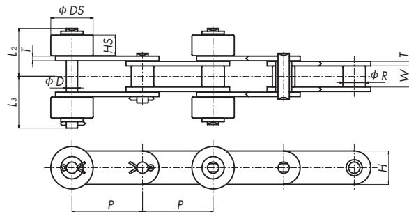
Crosswise Installation (Type II)
