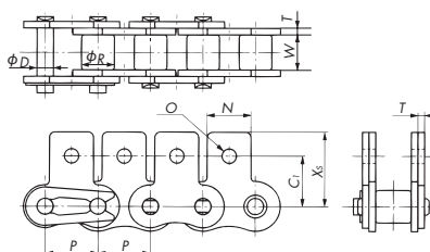
SK1 Attachment
