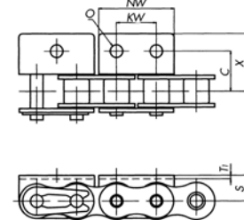
WA1, WA2 Attachments
