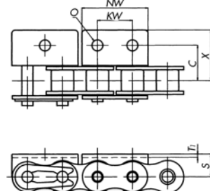
WA1, WA2 Attachments
