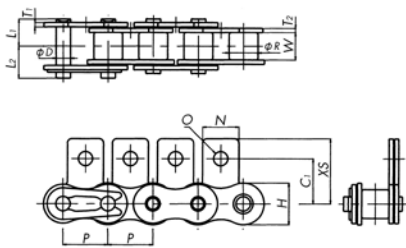
SA1 Attachment
